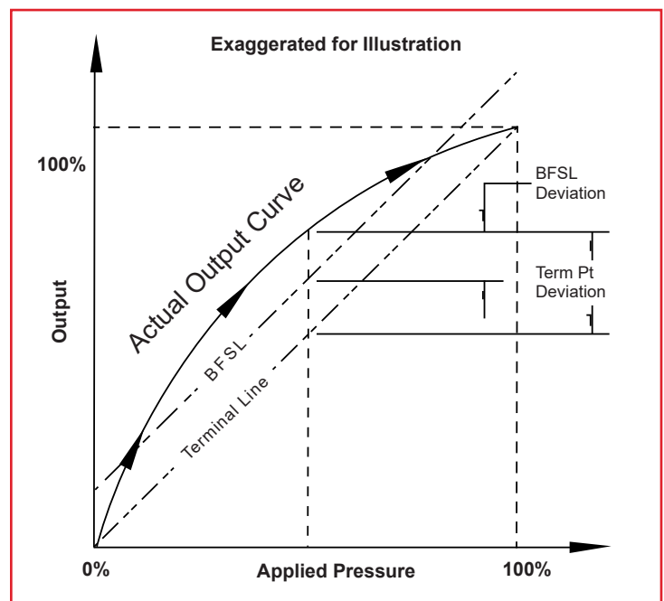
Figure 3: Non-Linearity Illustration
