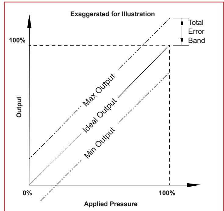
Figure 8: Total Error
