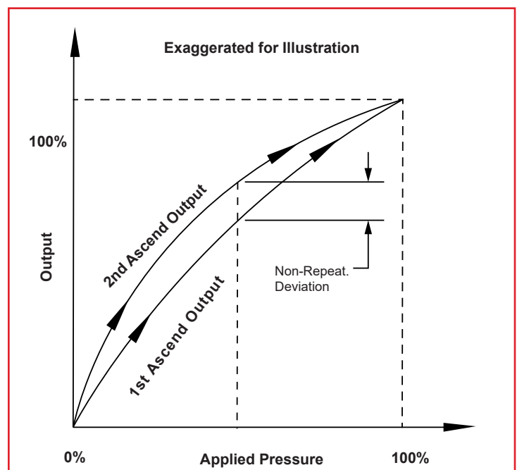
Figure 5: Non-Repeatability Illustration
