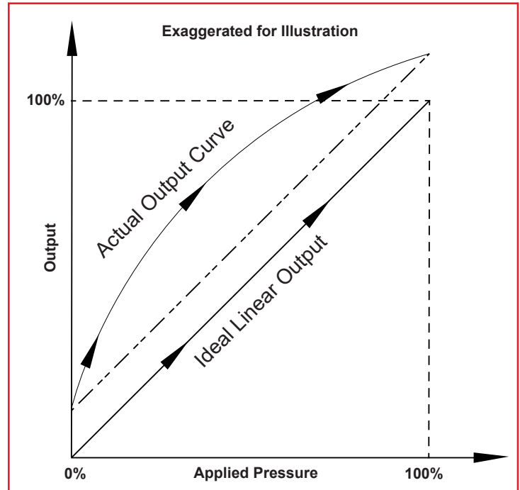
Figure 1: Actual Output vs. Ideal Output
