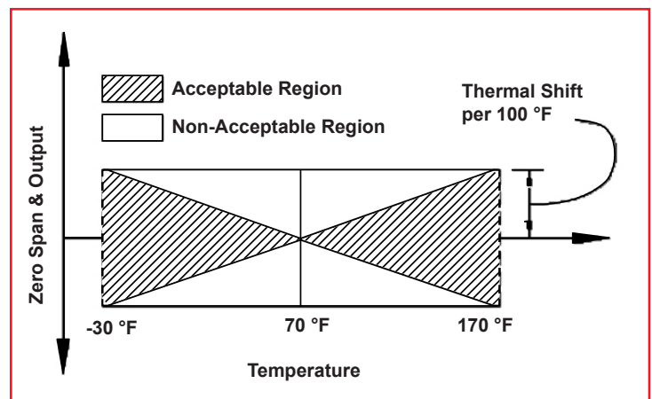
Figure 6: Thermal Zero & Span Shift
