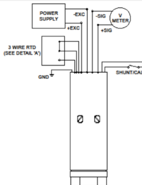
SHUNT CAL OPTIONS: GH, ME or NC WITH ADDITIONAL RTD OUTPUT
