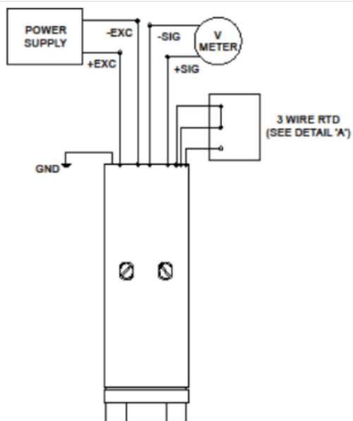
STANDARD WITH ADDITIONAL RTD OUTPUT
