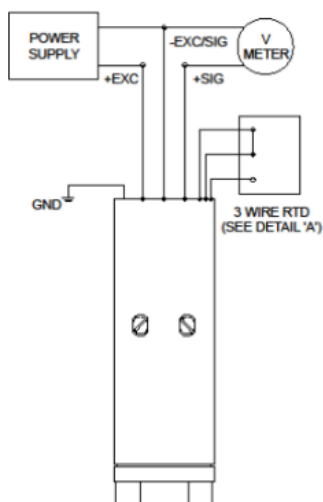
STANDARD WITH ADDITIONAL RTD OUTPUT
