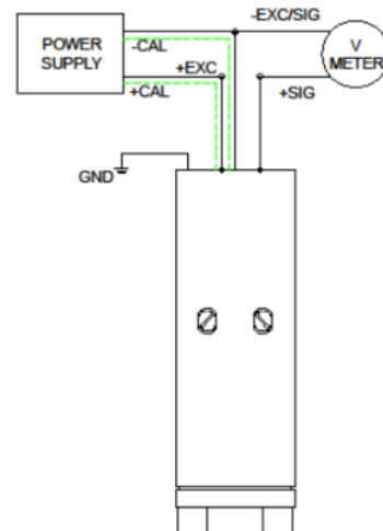
POWERED SHUNT CAL OPTION: NB (SHUNT ONLY ON VOLT OUTPUT)
