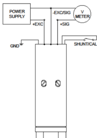
SHUNT CAL OPTIONS: GH, ME or NC (SHUNT ONLY ON VOLT OUTPUT)
