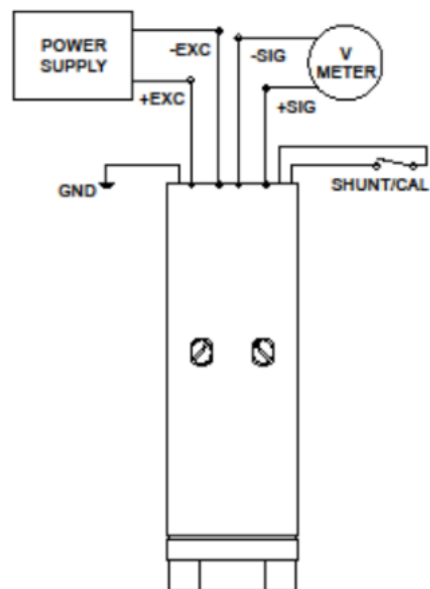
SHUNT CAL OPTIONS: GH, ME or NC
