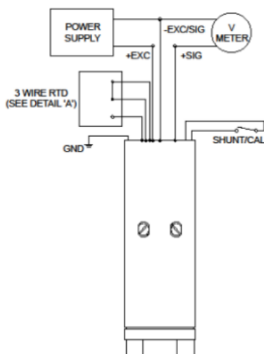
SHUNT CAL OPTIONS: GH, ME or NC WITH ADDITIONAL RTD OUTPUT
