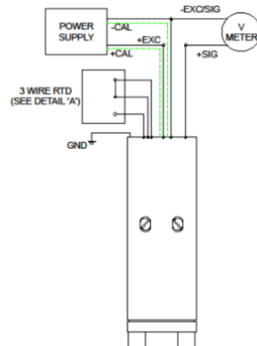
POWERED SHUNT CAL OPTION: NB WITH ADDITIONAL RTD OUTPUT
