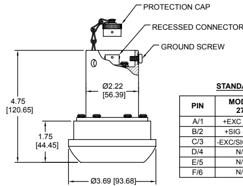
2" #1502 CONFIGURATION (SHOWN WITH "CA" CONNECTOR)
