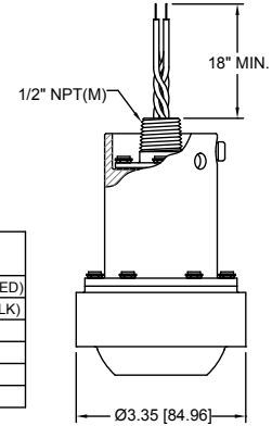
2" #2002/2202 CONFIGURATION (SHOWN WITH "CF" CONNECTOR)
